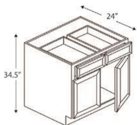
BASE CABINET: 2 Doors, 2 Drawers
